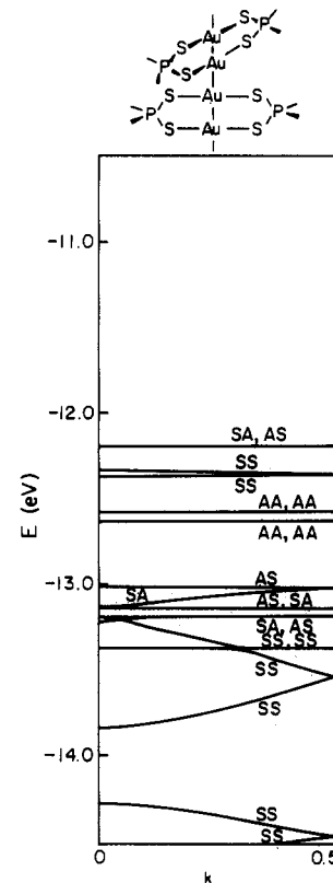
Figure 9. Band diagram for the staggered form of the polymer [\text{Au}_2(\text{S}_2\text{PH}_2)_2]_n .
